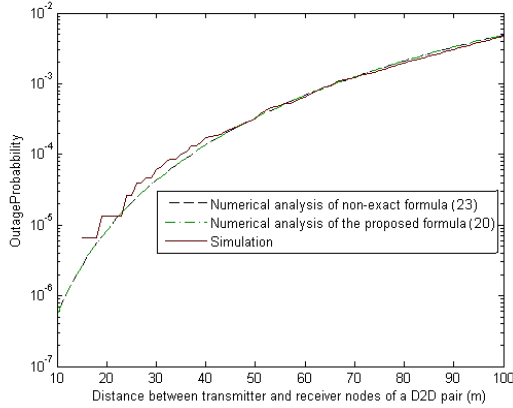
Fig. 3. Outage probability vs. the distance between the transmit and receive nodes of a D2D pair for underlay scenario
